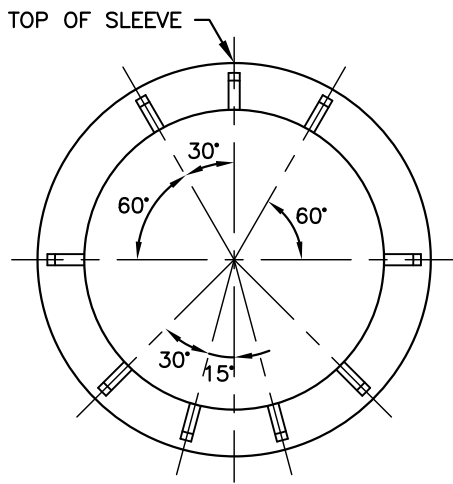
SPACER LOCATION FOR 16" THRU 36" DIA. CARRIER PIPE
