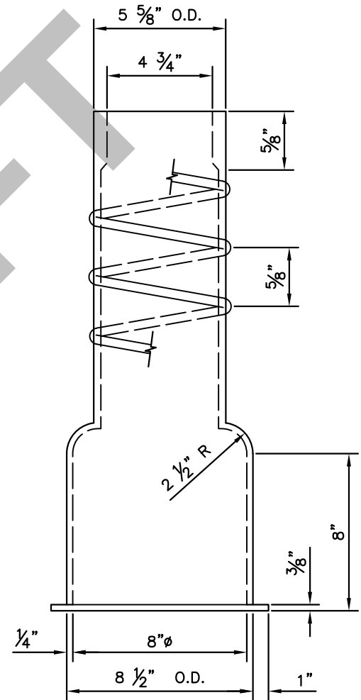
BOTTOM PROFILE
