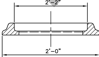
24" VAULT FRAME & COVER
