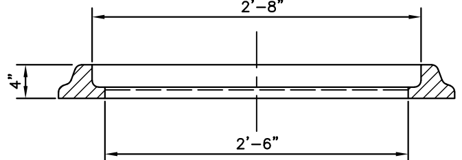
30" VAULT FRAME & COVER
